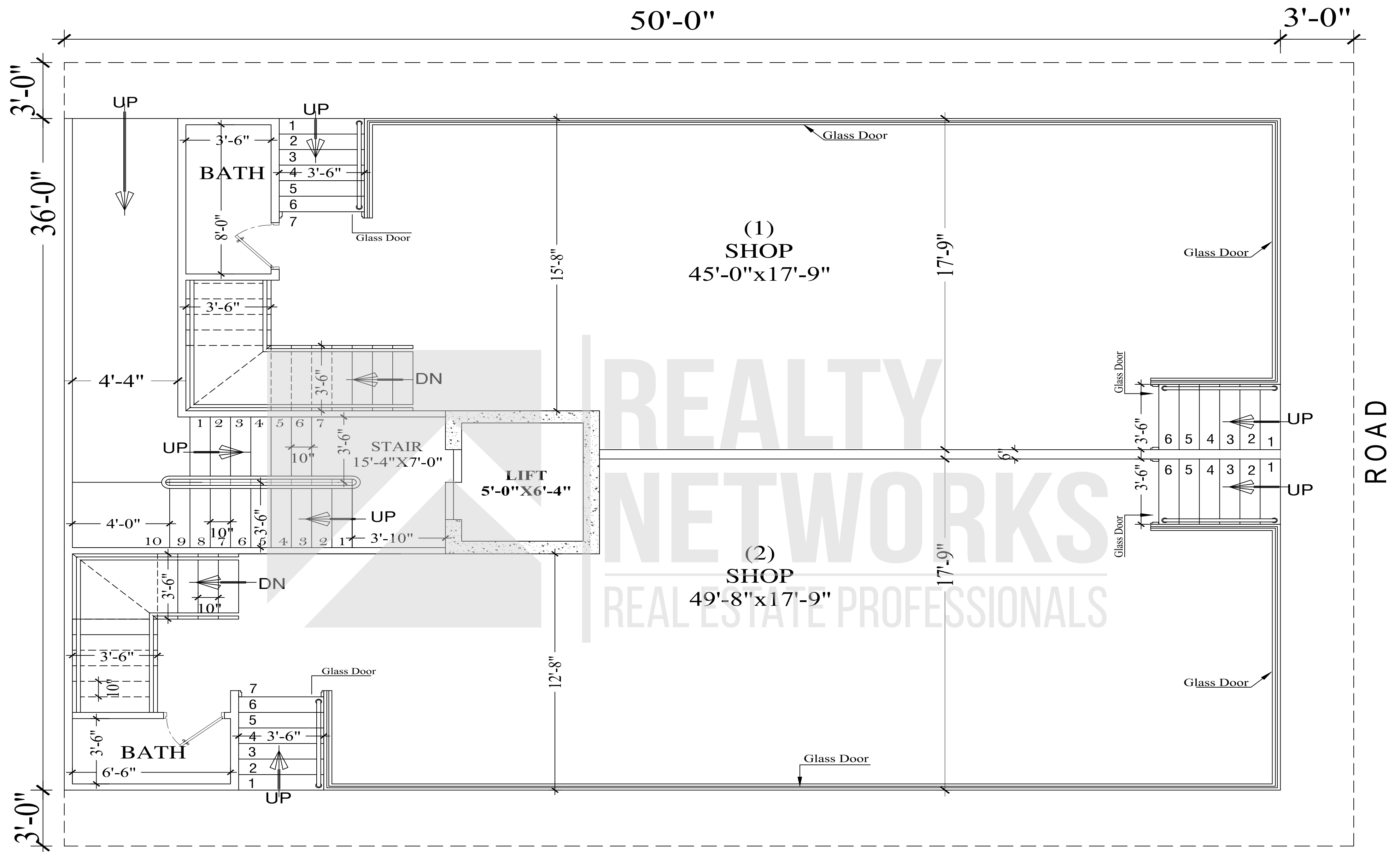
GROUND FLOOR PLAN OP-02
